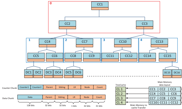
Figure 3: Proposed vEb memory integrity tree structure
