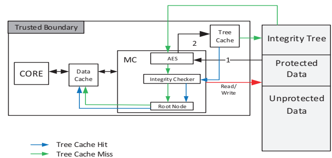
Figure 1: Security design model
