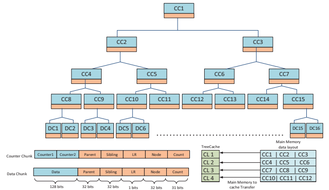
Figure 2: Standard memory integrity tree structure
