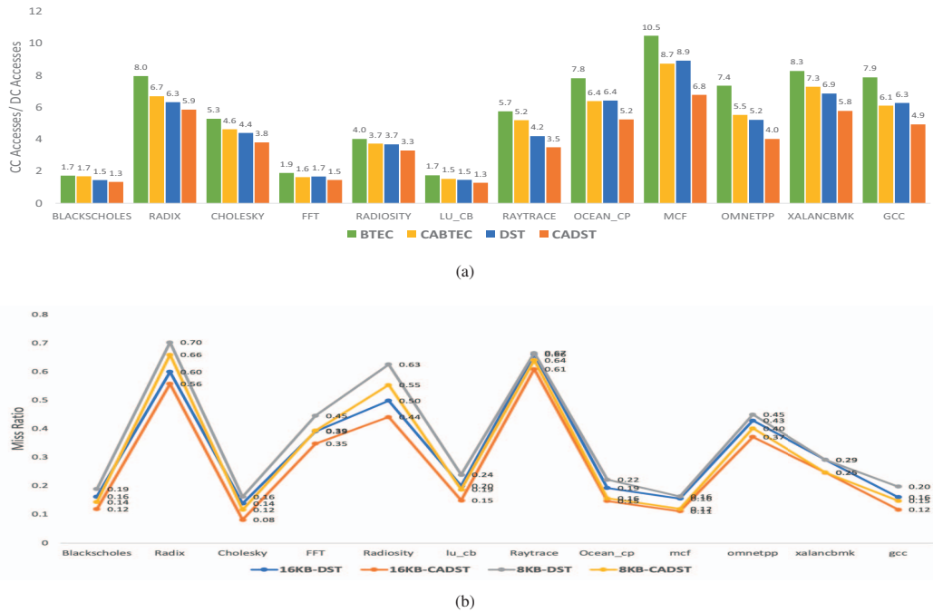
Figure 5: a) CCs per DC accessed, b) TreeCache miss ratio
