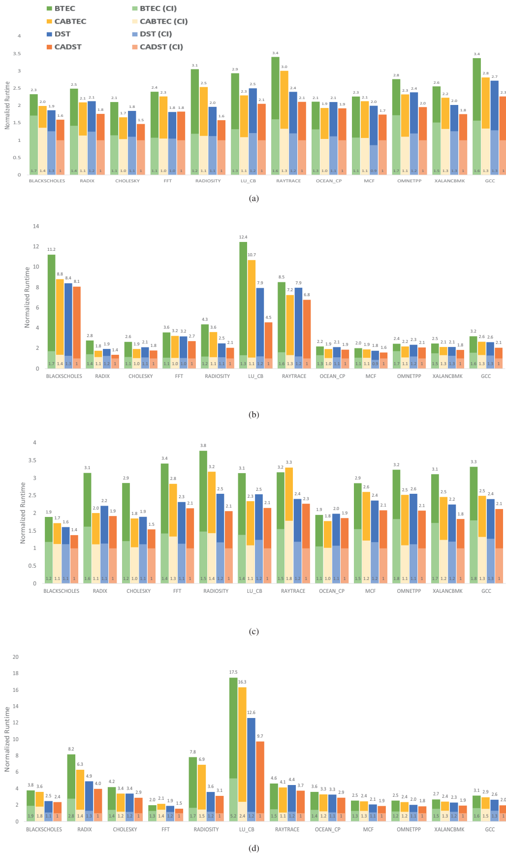
Figure 6: Run time for memory authentication with a) 16KB TreeCache, 64B cache line, b) 16KB TreeCache, 128B cache line c) 8KB TreeCache, 64B cache line d) 8KB TreeCache, 128B cache line 407
